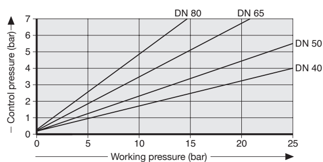
Actuator 125 (DA), flow below the seat
